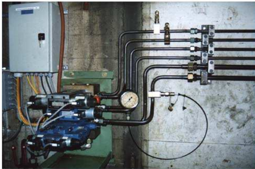
Picture 1: Pressure measurement with serv-Clip-1 of a servo- hydraulic system
